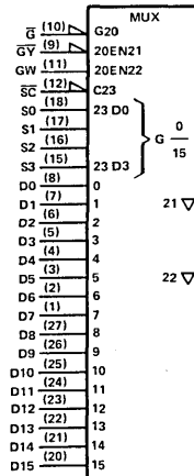
logic symbol† AS851
