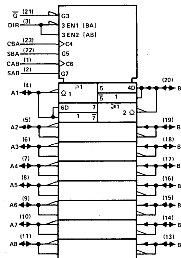
logic symbol, 'ALS649, 'LS649†
