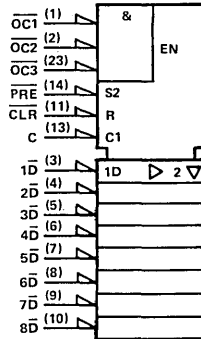
logic symbol
