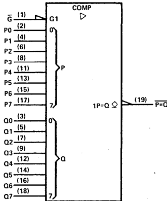
logic symbol, 'ALS689, 'LS689†
