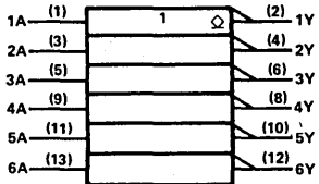
logic symbol†
