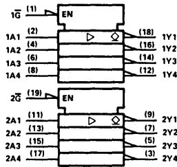
logic symbol 'AS762†
