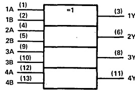
logic symbol, 'LB86†
