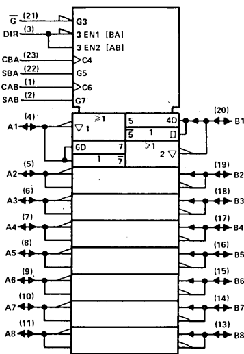
logic symbol, 'ALS648, 'AS648, 'LS648†
