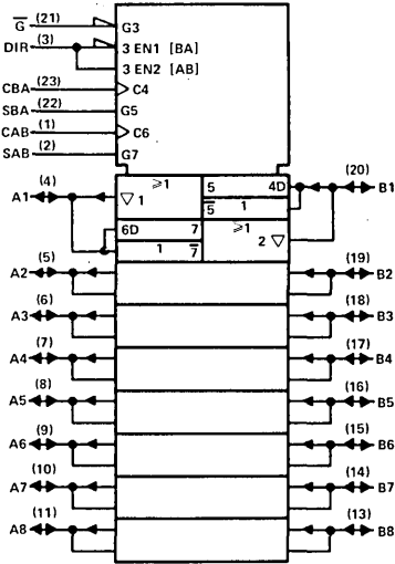
logic symbol, 'ALS646, 'AS646, 'LS646†
