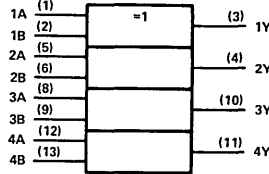
logic symbol, 'LB86†
