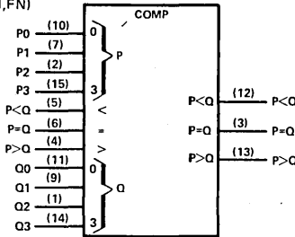
logic symbol, 'L85†
