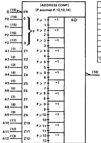
logic symbol, 'ALS679†
