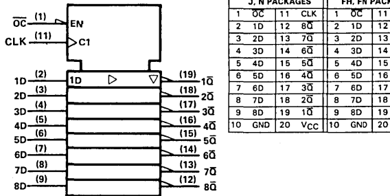
logic symbol†
