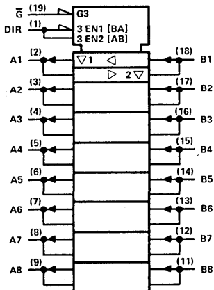
logic symbol† 'AS2640
