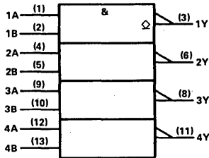
logic symbol†
