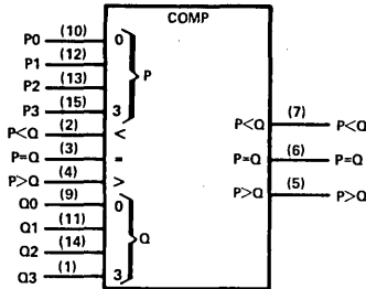
logic symbol, 'L85†
