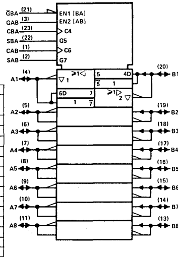
logic symbol, 'ALS652, 'AS652, 'LS652†
