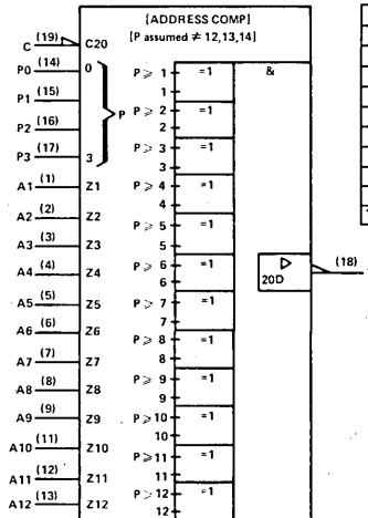
logic symbol, 'ALS680†
