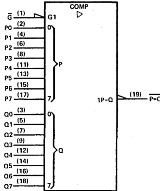
logic symbol, 'ALS688, 'LS688†
